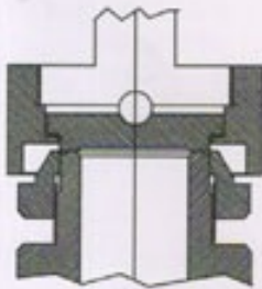
STANDARD DESIGN METAL TO METAL SEAT
