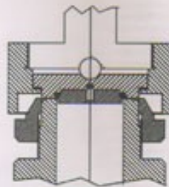
SOFT SEAT DESIGN FOR CRITICAL SERVICE
