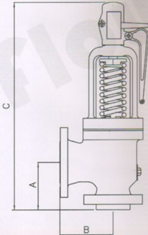
CLOSED CAP WITH PACKED LIVER FOR CONNOCNE MEDIA & LIQUID SERVICE PACKED LIVER
